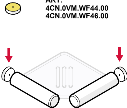
Bathroom shelf 400-NY and 400-SS
